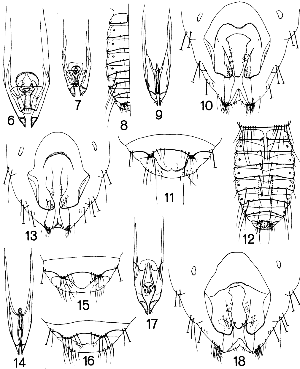
FIG. 6-18. 6, Psittaconirmus neumanni , ♂ genitalia. 7-8, P. johnstoniae : 7, ♂ genitalia; 8, ♂ dorsal abdomen. 9-12, P. hellenthalii : 9, ♂ genitalia; 10, ♀ ventral terminalia; 11, ♂ dorsal terminalia; 12, ♂ dorsal abdomen and metathorax margin. 13-15, P. zinki : 13, ♀ ventral terminalia; 14, ♂ genitalia; 15, ♂ dorsal terminalia. 16-18, P. charmosynae : 16, ♂ dorsal terminalia; 17, ♂ genitalia; 18, ♀ ventral terminalia.
