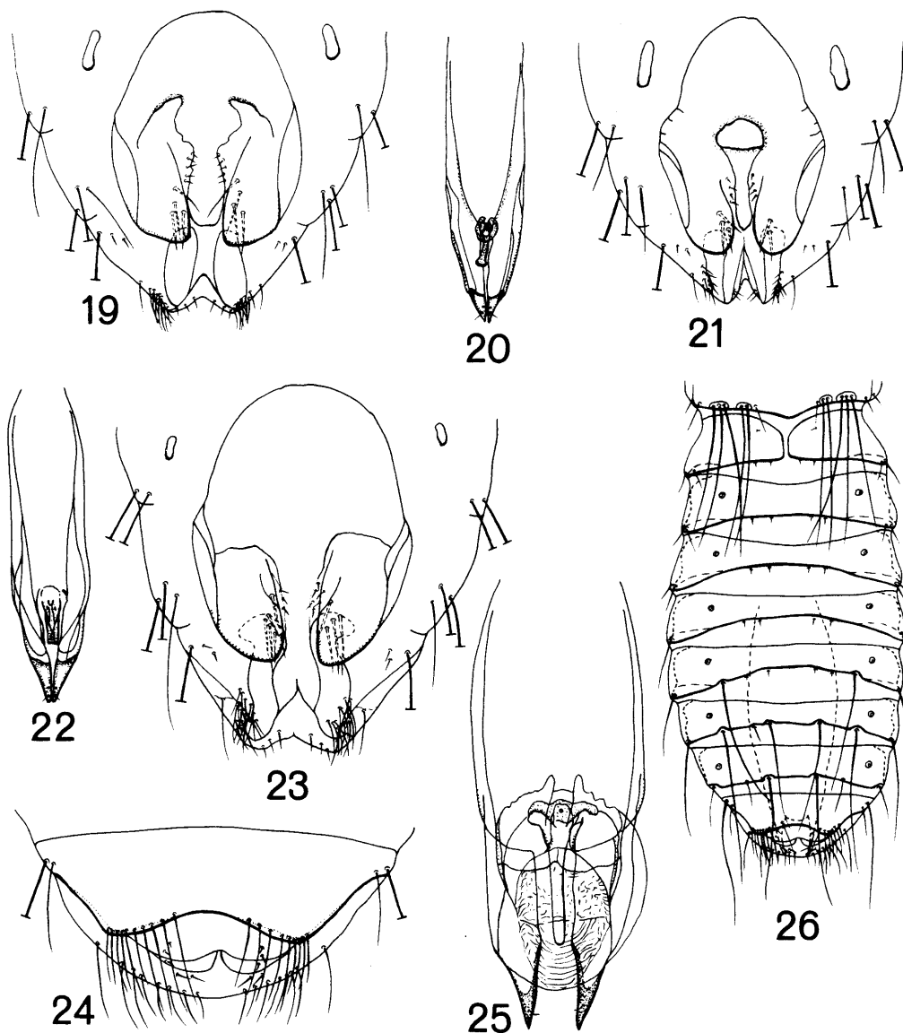
FIG. 19-26. 19-20, Psittaconirmus chlorocerci : 19, ♀ ventral terminalia; 20, ♂ genitalia. 21-22, P. comis : 21, ♀ ventral terminalia; 22, ♂ genitalia. 23-26, P. cardinalis : 23, ♀ ventral terminalia; 24, ♂ dorsal terminalia; 25, ♂ genitalia; 26, ♂ dorsal abdomen and metathorax margin.
